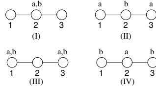
Fig. 2. Nash equilibrium channel assignment cases in any time slot. (The 'a' or 'b' denotes the channel(s) that the player assigns its radios to.)
