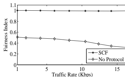
Fig. 4. Fairness index. ( |C| = 3, K = 2, R = 11Mbps. )
