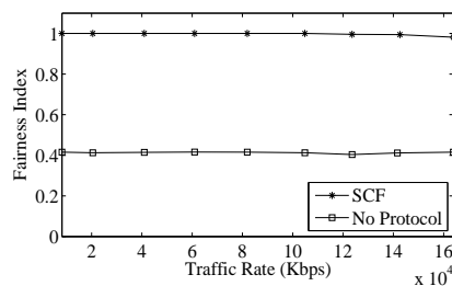
Fig. 5. Fairness index. ( |C| = 12, K = 4, R = 54Mbps. )
