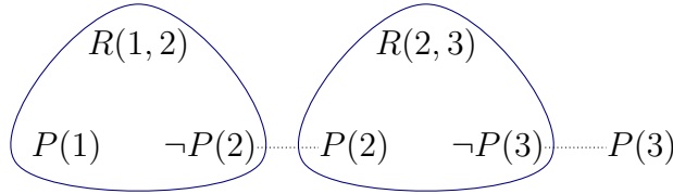
Fig. 4. The extended conflict hypergraph for I and F from Example 4.
